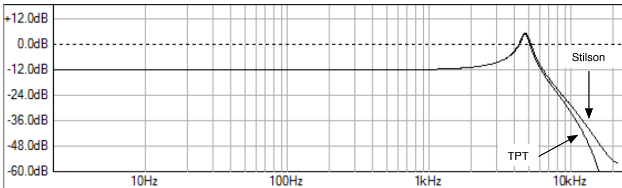
Figure 4.23: comparing the TPT and Stilson Ladder filters while holding resonant peaking and frequency constant shows differences only in the frequencies very close to Nyquist; the TPT version has the correct f_c and the Stilson version was adjusted until the peaks touched.
