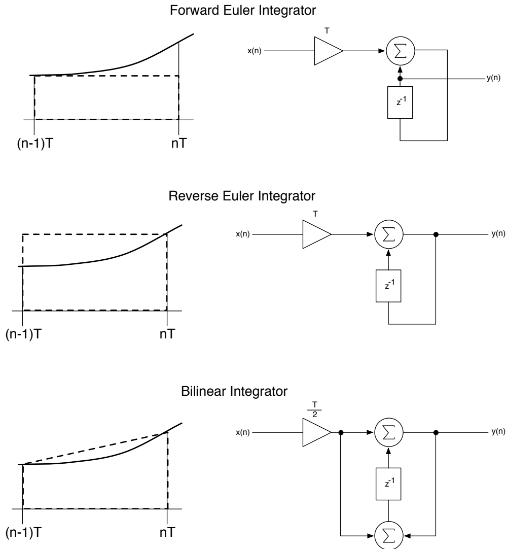
Figure 4.2: Several digital integrators with area of integration shown in dashed lines
