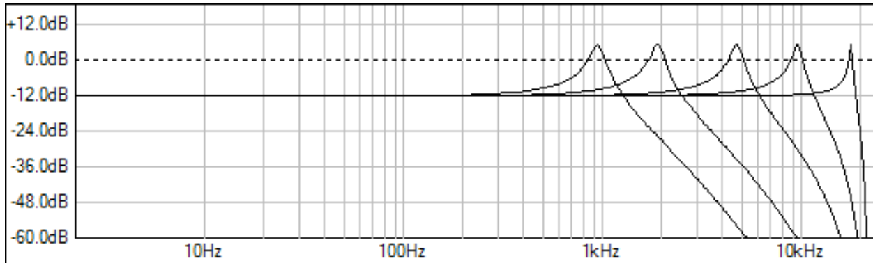
Figure 4.22: the responses for Q = 20 and f_c = 1\text{kHz}, 2\text{kHz}, 5\text{kHz}, 10\text{kHz}, and 18\text{kHz} .
