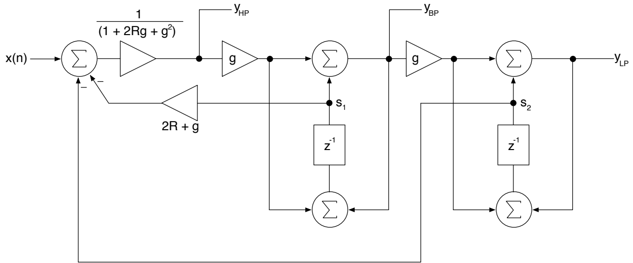
Figure 4.6: the TPT version of the SVF filter, the zero-delay loop has been resolved.
