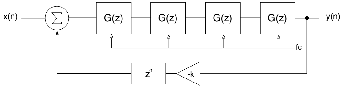
Figure 4.15: the Stilson-Smith implementation uses a delay in the feedback path
